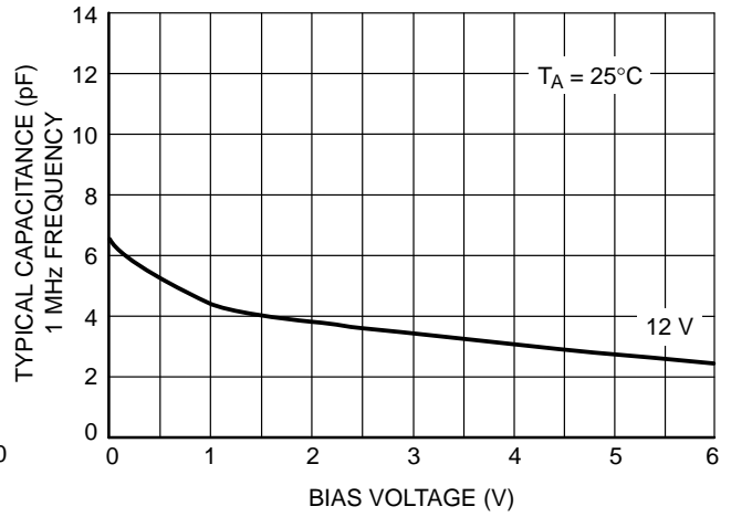
Figure 2. Capacitance
